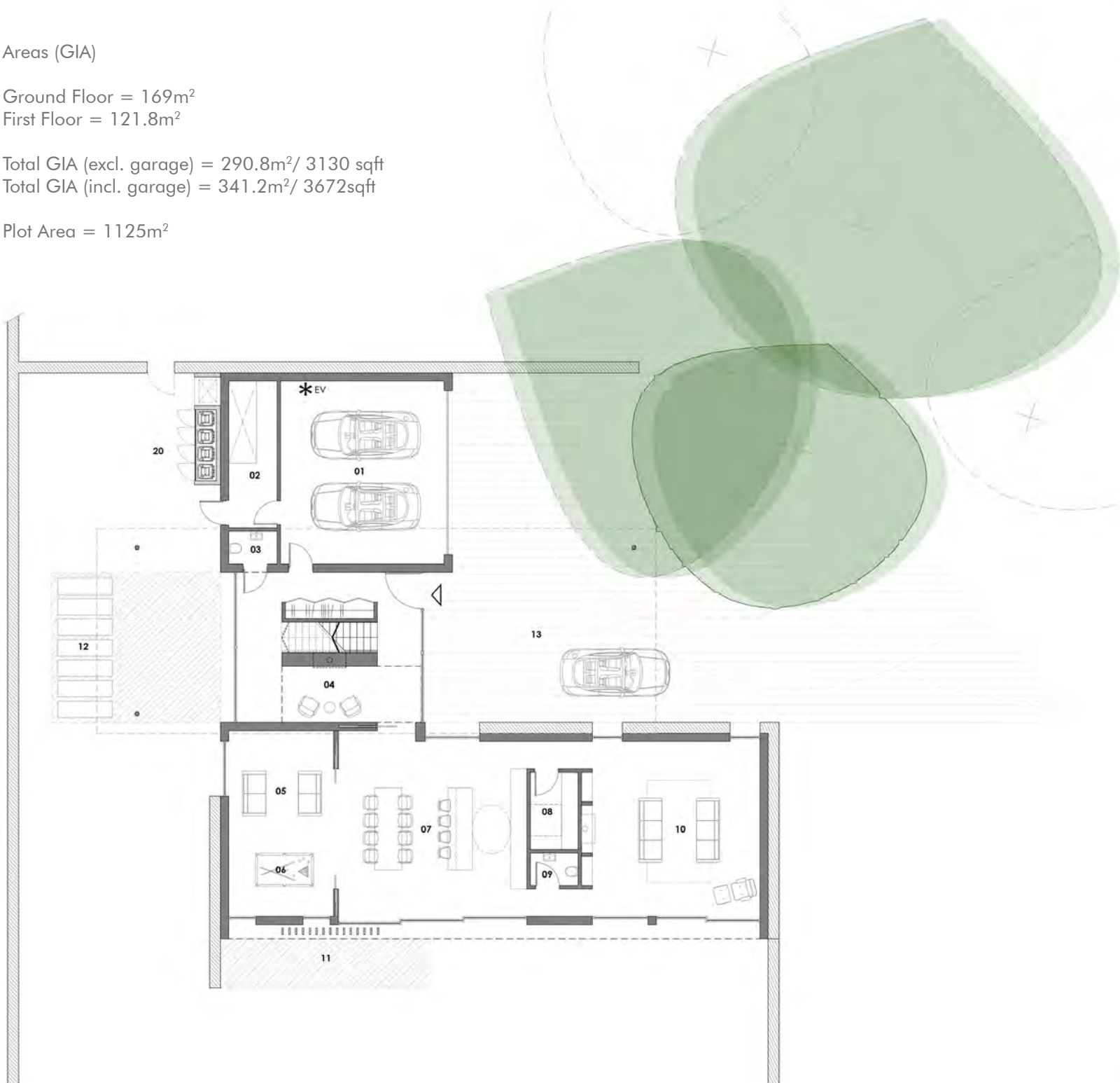
01 - Ground Floor
