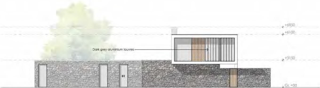
04 - North West Elevation
