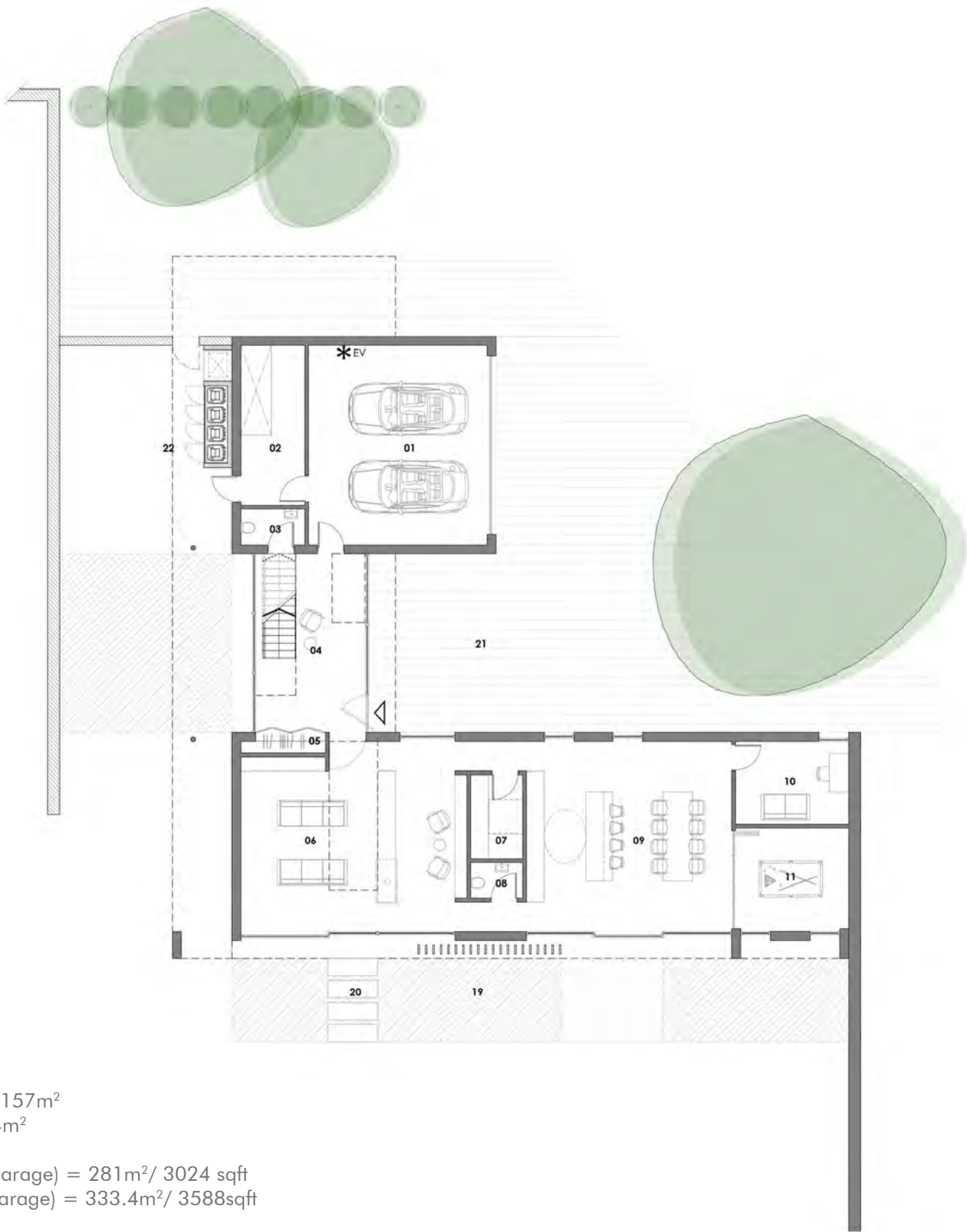
01 - Ground Floor
